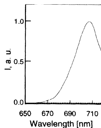
Figure 2. Luminescence spectra (room temperature, DMF solution, \lambda_{\text{exc}} 494\text{nm} ) of 3 (—, [\mathbf{3}] = 1.0 \times 10^{-6}\text{M} ) and 2 + \text{Ru}(\text{MePh-tpy})_2^{2+} (-----, [\mathbf{2}] = 1.0 \times 10^{-6}\text{M} , [\text{Ru}(\text{MePh-tpy})_2^{2+}] = 1.0 \times 10^{-4}\text{M} ).
