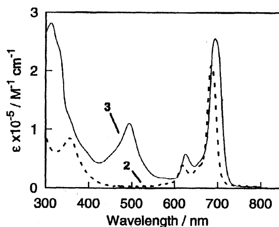
Figure 1. Absorption spectra (room temperature, DMF solution) of 2 and 3 .
